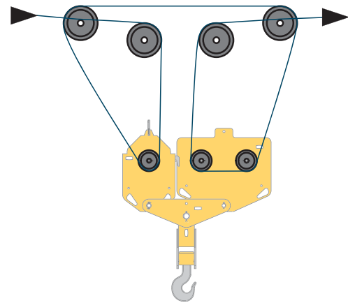
2C 4-fall rope reeving
