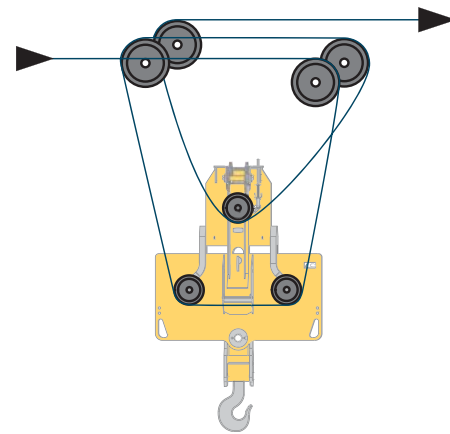
SM/DM 4-fall rope reeving
