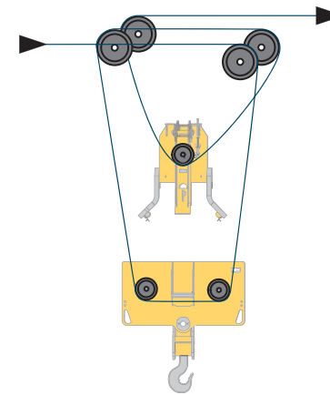
SM/DM 2-fall rope reeving
