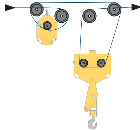
2C 2-fall rope reeving
